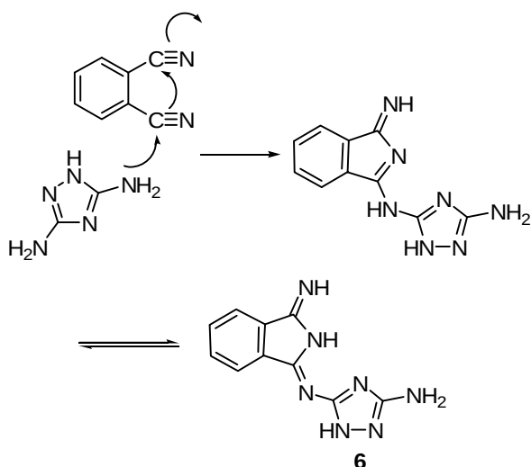
Scheme 2. The mechanism of the formation of a triazolehemiporphyrazine starting from a phthalonitrile precursor.
