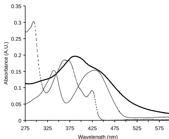
Figure 2. UV-vis spectra of hemipyrazinoporphyrazine 8b (thick solid line), a typical triazolehemiporphyrazine ( 3 , R = C_{12}H_{25} , R' = OC_8H_{17} , M = Ni , dotted line), and 5,6-bis(1 H -pyrrol-2-yl)-pyrazine-2,3-dicarbonitrile ( 5 ) (thin solid line) in DMF.
