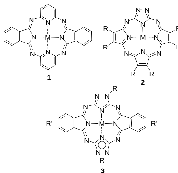
Figure 1. Chemical structures of hemiporphyrazine ( 1 ), triazoleazaporphyrin ( 2 ) and triazolehemiporphyrazine ( 3 ).
